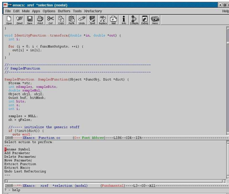
Figura 3.3: XRefactory
